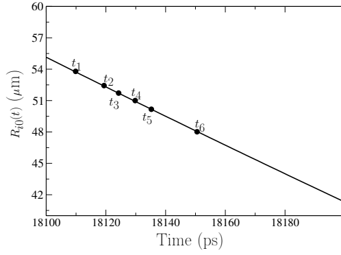
Figure 15: Time evolution of the Lagrangian radius r_{i_0}(t) associated to the spatial mesh where the \alpha -suprathermal component represented in Fig. 16 is calculated. The observation times corresponding to the sequence shown in Fig. 16 have also been indicated.
