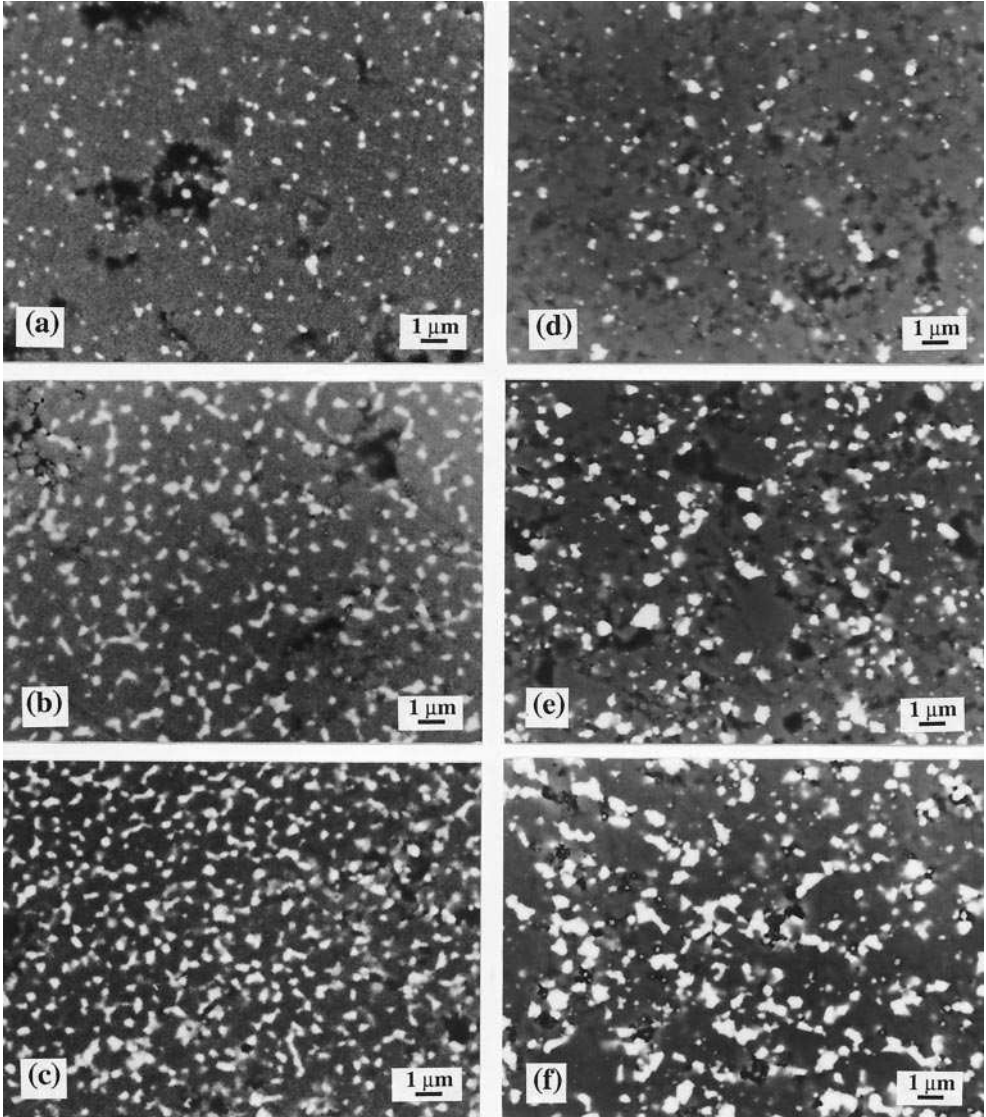
Fig. 5. SEM back-scattered images (BEI) of the polished surface of the hot-pressed \text{ZrO}_2 - \text{MgAl}_2\text{O}_4 composites (a) BM5, (b) BM20, (c) BM30, (d) A5, (e) A20, and (f) A30.
