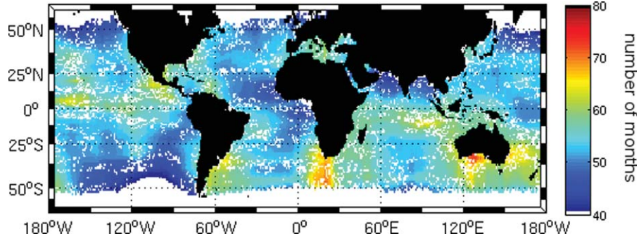
Figure 6. Estimated duration of needed Sentinel 3-OLCI month measurements to enhance the joint SeaWiFS-MERIS detection of long-term linear trend: from simulations of model (equation (9), see text for details).
