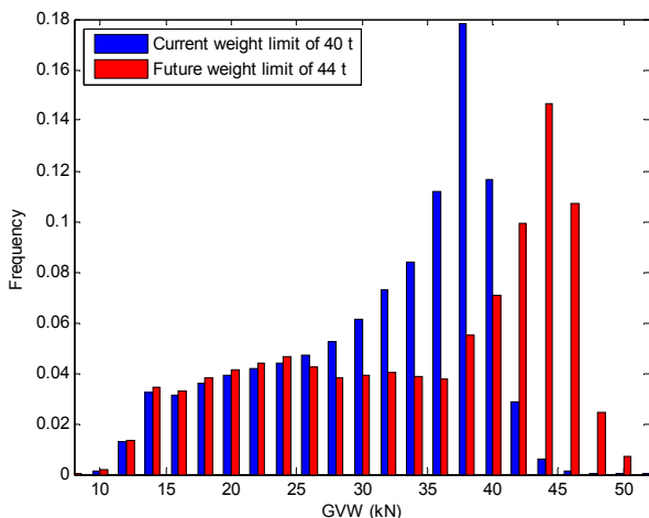
Figure 10. Comparison of 5-axle truck GVW histogram under current and future weight limit.
