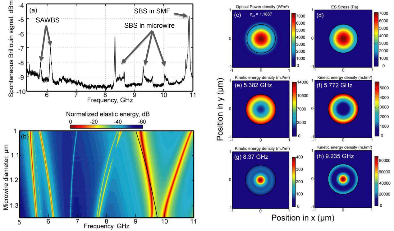
Figure 1: (a) Experimental Brillouin scattering spectrum measured at 1.55 \mu\text{m} in 8-cm long silica optical microfiber with a waist of 1 \mu\text{m} and for a CW pump power of 100 \text{ mW} . (b) Computed elastic energy of phonon wave packet (i.e., the theoretical Brillouin spectrum) versus the acoustic frequency and for a microwire waist varying from 1 \mu\text{m} to 1.35 \mu\text{m} . The black line shows the SBS phase-matching condition ( K=2K_p ). (c-g) Numerical results for a 1.05 \mu\text{m} silica rod diameter. (c) Optical power in the fundamental TE-like mode at a wavelength of 1.55 \mu\text{m} ( n_{\text{eff}} = 1.1887 ). (d) Spatial distribution of the electrostrictive force with 1 \text{ W} optical power. (e,f) Elastic energy density of resonant surface acoustic waves at 5.382 \text{ GHz} and 5.772 \text{ GHz} , respectively. (g,h) Elastic energy density of longitudinal acoustic modes at 8.37 \text{ GHz} and 9.235 \text{ GHz} .
