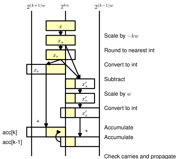
Fig. 3: Scalar accumulation scheme.
