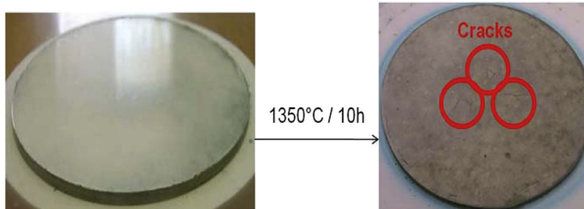
Fig. 9. Large-scale half-cell before and after sintering.
