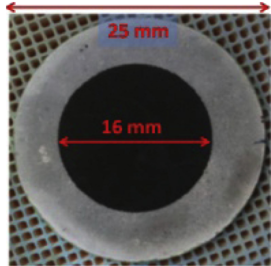
Fig. 3. Picture of a 25 mm cell.
