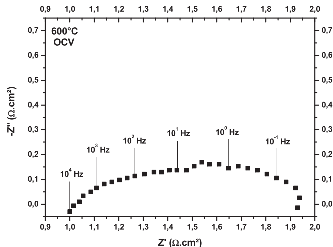
Fig. 12. Nyquist plots of a 40 mm Ni-BCY10/BCY10/Pr 2 NiO 4+δ single cell at 600 °C.
