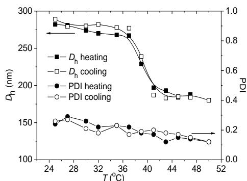
Fig. 5 Evolution of D_h and PDI of the GNR@PEG 114 - b -PNVCL 237 aqueous suspension (50 \mu g/mL) upon heating (solid) and cooling (open). The solid lines here just serve to guide the eyes.
