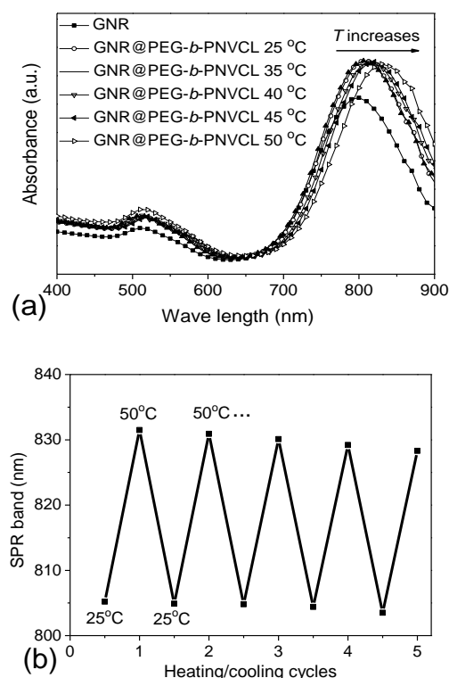
Fig. 6 UV/ vis adsorption spectra of the GNR@PEG 114 - b -PNVCL 237 aqueous suspension (50 \mu g/mL) under different temperatures (a); and evolution of longitudinal SPR band of the GNR@PEG 114 - b -PNVCL 237 aqueous suspension (50 \mu g/mL) during multiple cooling (25 °C)/heating (50 °C) cycles (b). The solid lines here just serve to guide the eyes.
