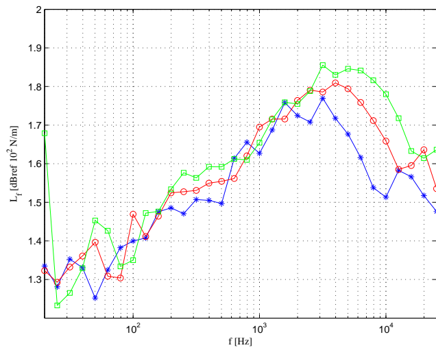
Figure A.14: 1/3 octave spectrum of the contact stress at point (x_0 = 0, y_0 = 0) for road (A) and for the velocities : -*- V_0 = 50 \text{ km/h} , -o- V_0 = 70 \text{ km/h} , -□- V_0 = 90 \text{ km/h} .
