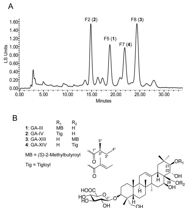
Figure 2. Purification and identification of gymnemic acids (GAs). (A) Solvent extracted and semi-purified GAs were fractionated on preparative HPLC (Sunfire C 18 5 \mu m, 250 \times 10 mm) using an isocratic mobile phase (see “Materials and Methods” for details). Fractions with major peaks were collected using an automated fraction collector, vacuum dried and assayed for inhibition of C. albicans yeast-to-hypha conversion. Individual fractions (F2, F5, F7 and F8) were evaluated for purity and molecular weight analyses using analytical HPLC-ELSD-DAD-MS, ESIMS, HRESIMS, 1 H NMR and 13 C NMR (see Figures S1–S20). (B) The four gymnemic acids (1–4) were identified using mass and NMR data (see Figures S1–S20 for details of GA species) according to Liu et al. [35] and Yoshikawa et al. [36,37,38]. The general structure of GA, methylbutyryl and tigloyl are shown. doi:10.1371/journal.pone.0074189.g002
