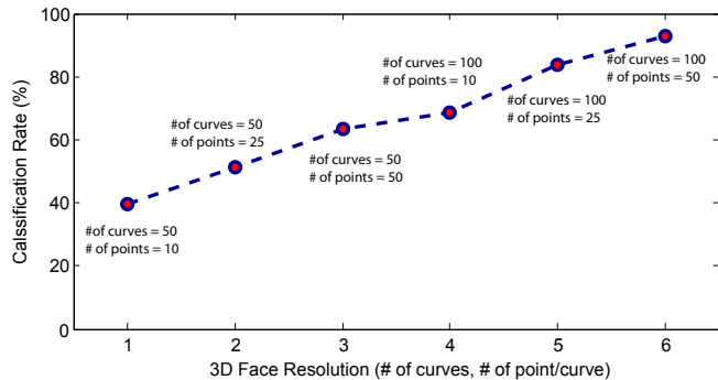
Fig. 14. Effects of varying the 3D face resolution on the classification results.
