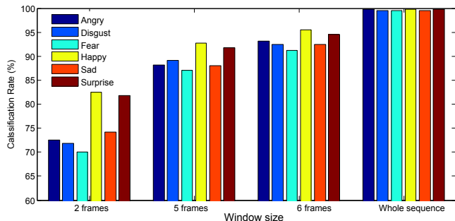
Fig. 13. Effect of the temporal size of the sliding window on the results. The classification rates increase when increasing the length of the temporal window.
