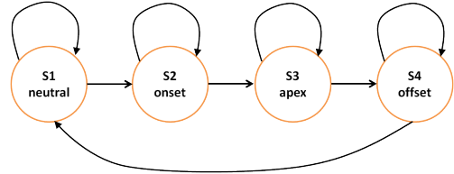
Fig. 8. Structure of the HMMs modeling a 3D facial sequence. The four states model, respectively, the neutral , onset , apex and offset frames of the sequence. As shown, from each state it is possible to remain in the state itself or move to the next one (this is known as Bakis or left-right HMM).
