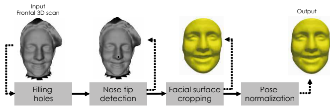
Fig. 10. Outline of the preprocessing steps. A pipeline of four filters is applied to each 3D sequence: (i) Filling holes, if any; (ii) Nose tip detection (for the first frame) and tracking (for remaining frames); (iii) Face cropping using a sphere centered on the nose tip and of radius 90mm; (iv) Pose normalization based on the ICP algorithm.
