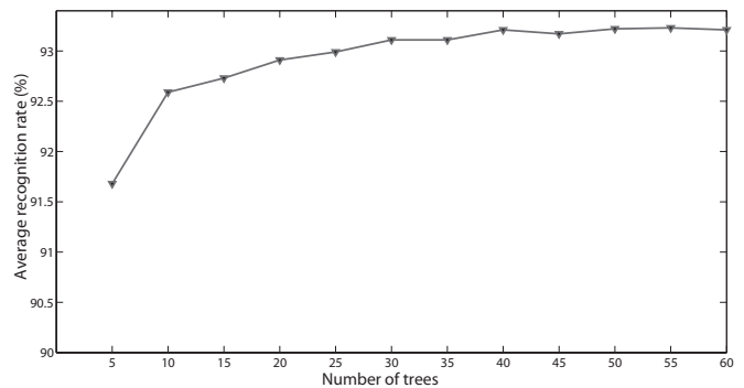
Fig. 12. 4D expression recognition results using a Random Forest classifier when varying the number of trees.
