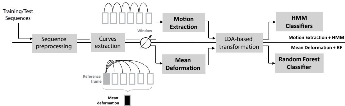
Fig. 1. Overview of the proposed approach. Four main steps are shown: Sequence preprocessing and extraction of the radial curves; Motion extraction and Mean deformation computation; Dimensionality reduction with LDA; HMM- and Random-Forest-based classification. Note that both train and test sequences can go through the upper and lower path in the block-diagram.
