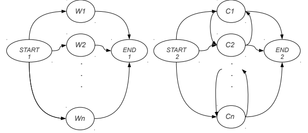
Fig. 2. a word network (a) a character network (b).
