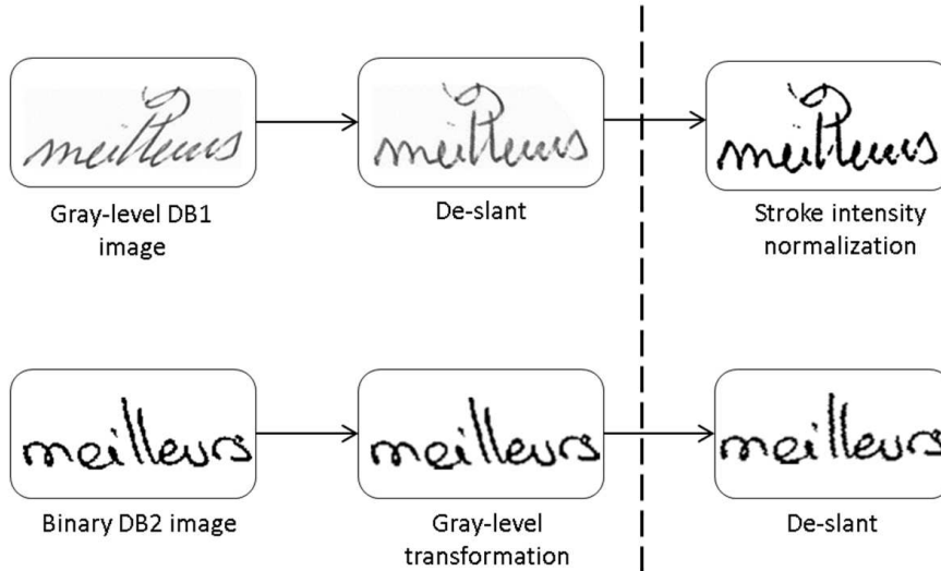
Figure 3. Training database adaptation through stroke intensity normalization
