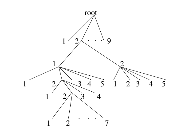
Fig. 12. Splitting a Linearized Thesaurus
