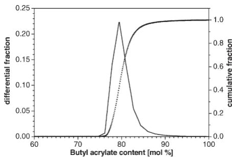
Figure 8. Differential (solid line) and cumulative (triangles) BA distributions in mol % of sample No. 32.
