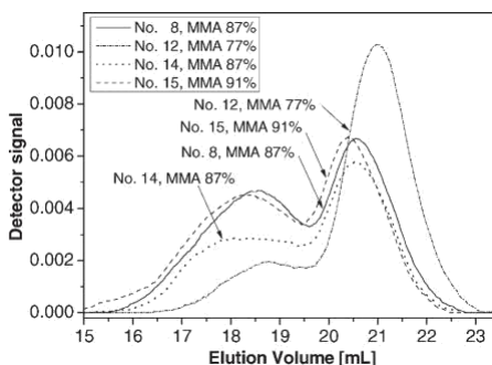
Figure 3. Overlay of the chromatograms of EMMA copolymer samples, as obtained by SEC.
