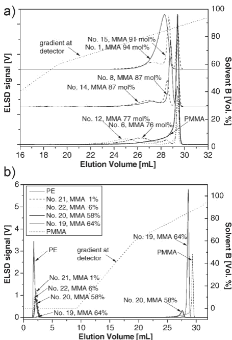
Figure 5. Overlay of chromatograms of EMMA samples: a) with isolated ethylene units and short ethylene sequences b) multiblock copolymer samples. Stationary phase: Perfectsil 300. Mobile phase: TCB and gradient TCB ! cyclohexanone/TCB (80/20 v/v). Temperature: 140 °C. Gradient at the ELSD is indicated by a dotted line.
