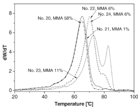
Figure 1. Overlay of curves obtained by CRYSTAF for EMMA samples.
