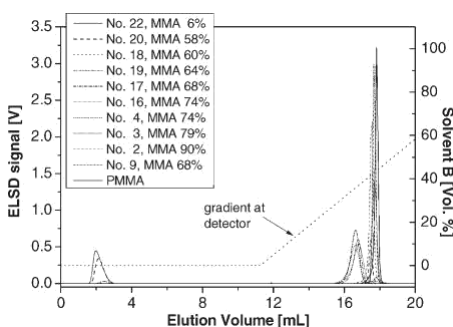
Figure 4. Overlay of the chromatograms of EMMA copolymer samples. Stationary phase: Perfectsil 300. Mobile phase: TCB and gradient TCB ! cyclohexanone. Temperature: 140 °C. Notice: the gradient at the ELSD is indicated in dotted line.
