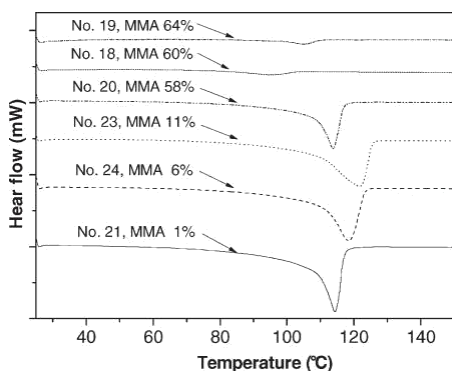
Figure 2. Overlay of DSC second heating curves of EMMA samples.
