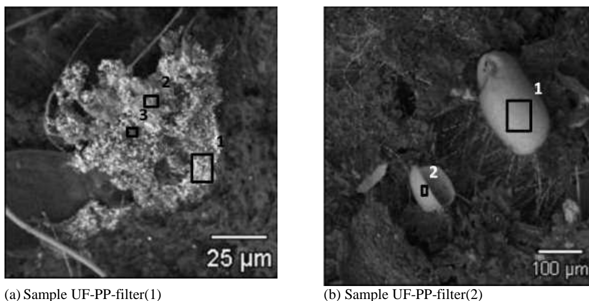
Figure 8 SEM-BSE images of the filter surface through which the effluent from the UF-PP column was passed
