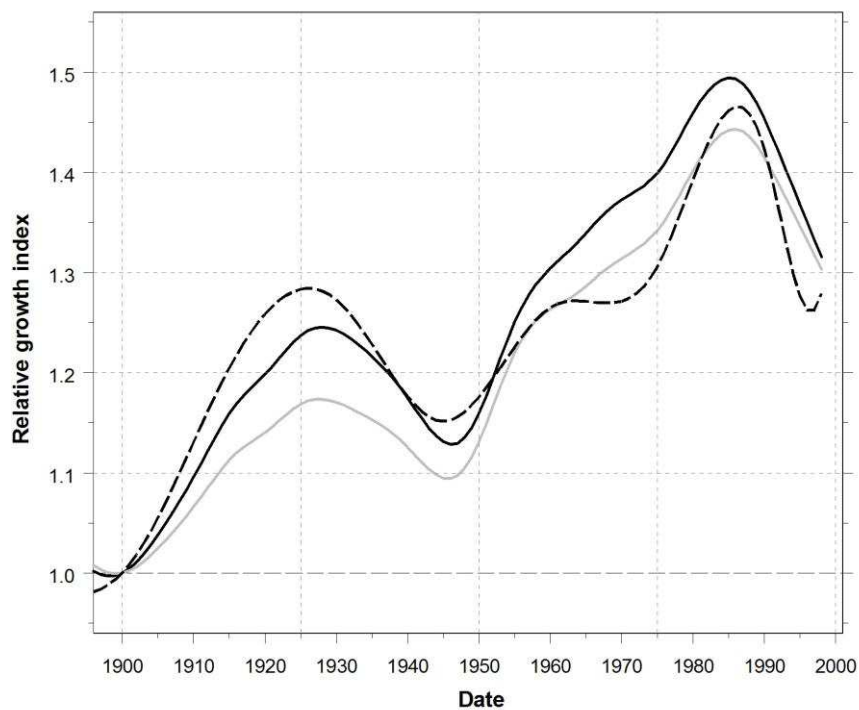
Figure 3. Comparison of radial growth chronologies estimated by the RCS (Regional Curve standardisation) and SM (Statistical Modelling) methods.
