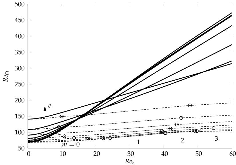
FIGURE 13. Absolute (solid lines) and convective (dotted lines) instability thresholds: critical Re_\Omega versus Re_z , for e = 0, 0.1, \dots, 0.7 . Open circles indicate a change of critical m for CI. For AI, the critical mode is always m = 0 .
