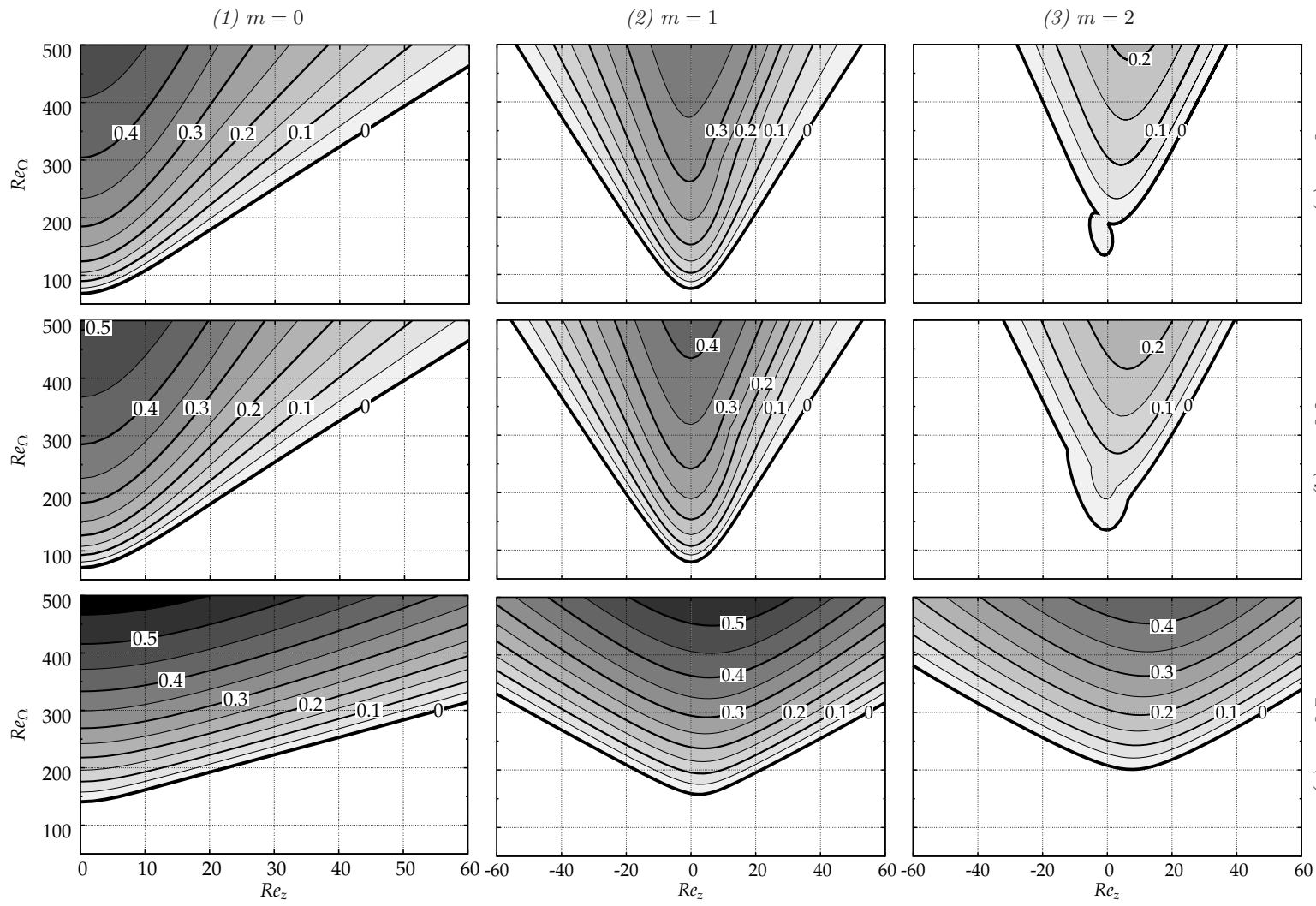
FIGURE 10. Absolute growth rate \omega_{0,i} maps for e = 0, 0.2, 0.7 , m = 0, 1, 2 .
