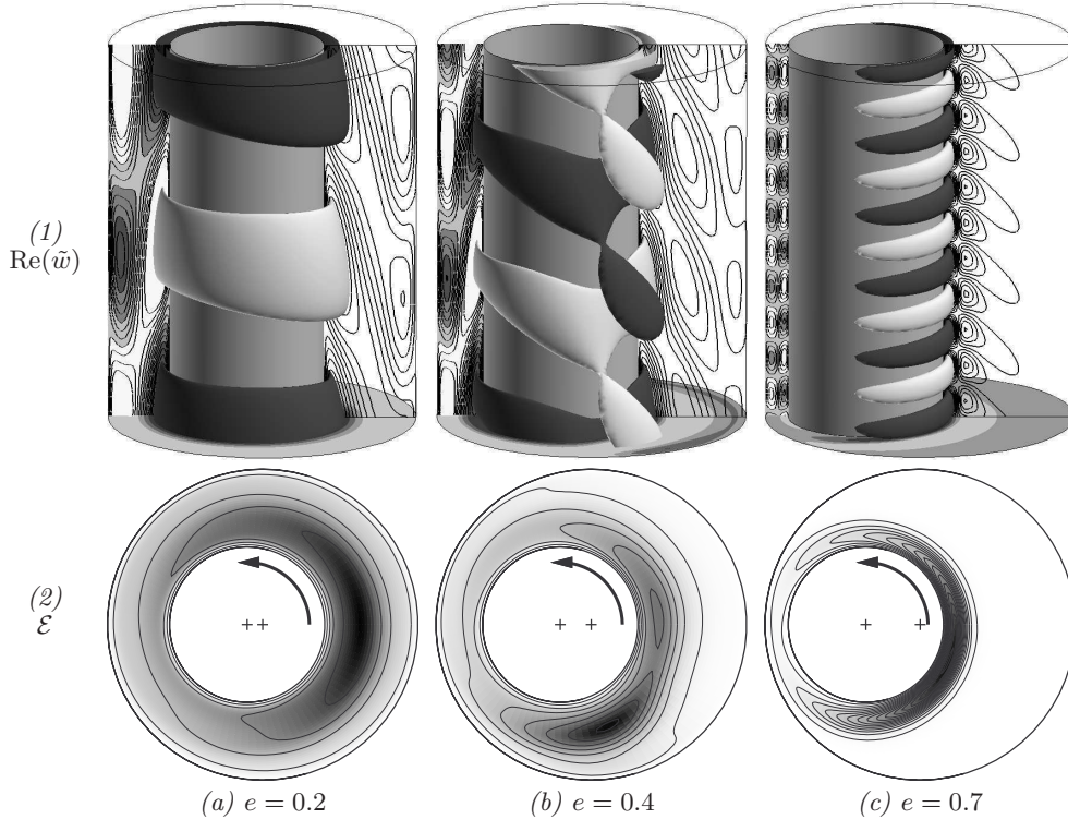
FIGURE 11. Critical mode m = 0 for Re_z = 60 , (a) e = 0.2 , Re_\Omega = 465.82 , (b) e = 0.4 , Re_\Omega = 432.74 , (c) e = 0.7 , Re_\Omega = 314.16 . (1) Distribution of axial perturbation velocity \text{Re}(\tilde{w}) . Dark (resp. light) grey is for positive (resp. negative) values. (2) Distribution of perturbation kinetic energy \mathcal{E} = \frac{1}{2}(\|\tilde{\mathbf{u}}_\perp\|^2 + |\tilde{w}|^2) . Dark grey indicates high values, and isocontours are equispaced.
