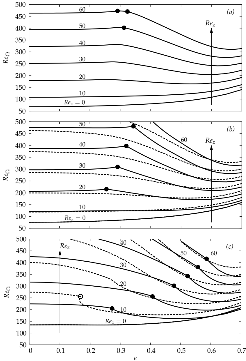
FIGURE 8. Critical azimuthal Reynolds number Re_\Omega versus eccentricity e for (a) m = 0 , (b) |m| = 1 and (c) |m| = 2 . Curves are drawn for Re_z = 0, 10, \dots, 60 . Solid lines are for m \geq 0 , and dotted lines for m < 0 . Filled/open dots indicate a change of saddle point.
