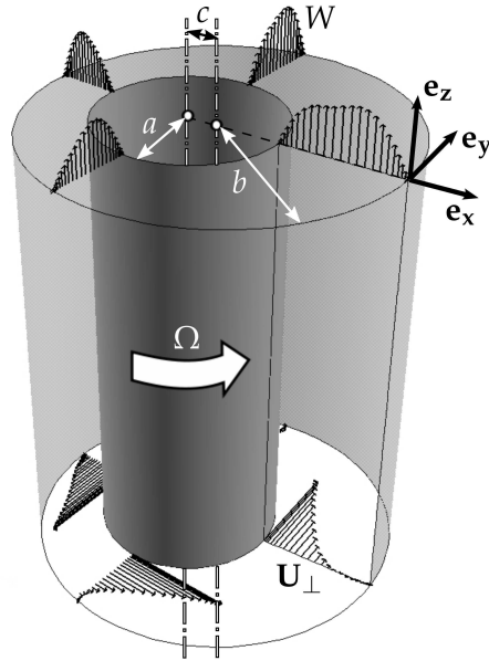
FIGURE 1. Eccentric annulus of radius ratio \eta = a/b = 0.5 and basic flow \mathbf{U} = \mathbf{U}_\perp + W\mathbf{e}_z .
