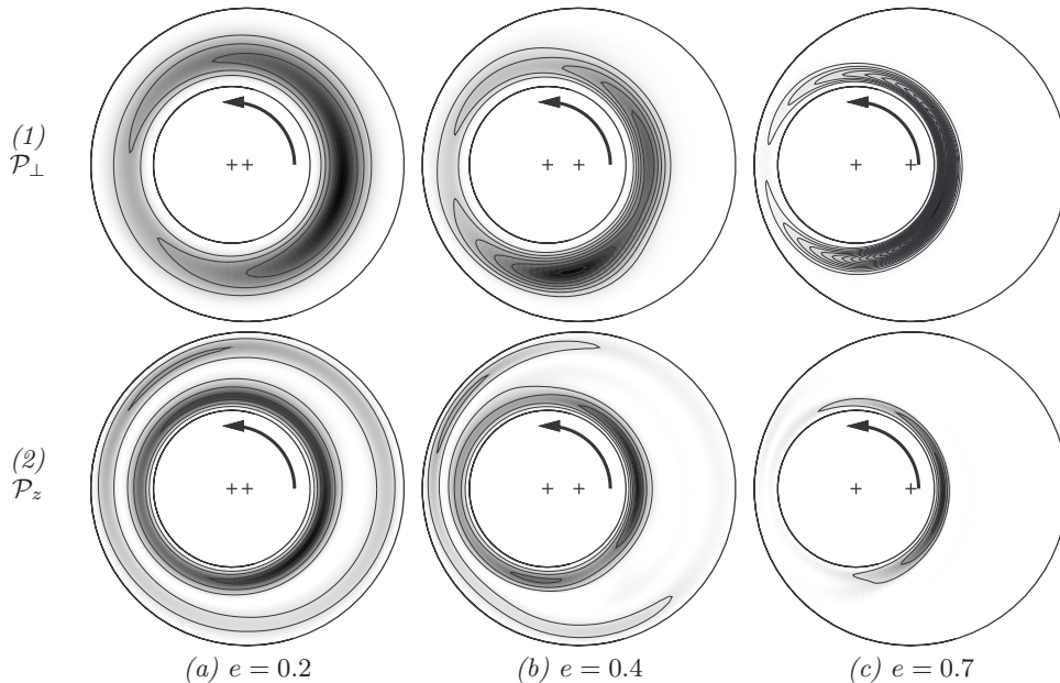
FIGURE 12. Distribution of kinetic energy production for m = 0 and Re_z = 60 , at critical conditions. (1) \mathcal{P}_\perp and (2) \mathcal{P}_z . (a) e = 0.2 , Re_\Omega = 465.82 , (b) e = 0.4 , Re_\Omega = 432.74 , (c) e = 0.7 , Re_\Omega = 314.16 . Dark grey indicates large contributions and white corresponds to zero or negative contribution. Isocontours are equispaced.
