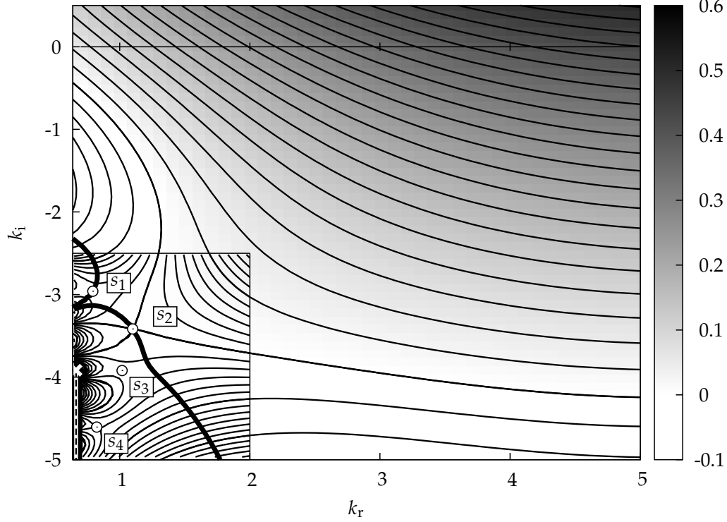
FIGURE 6. Contours of temporal growth rate at criticality for m = 0 , e = 0.3075 and Re_z = 60 ( Re_\Omega = 472.24 ). Saddles are indicated by white dots. The thick line indicates the steepest descent path associated with the pinch points s_1 and s_2 . The white cross indicates a branch point \partial k/\partial \omega = 0 from which originates a branch cut (vertical dotted line). The temporal growth rate of s_2 is larger than that of s_1 : the pinch s_2 dominates the impulse response.
