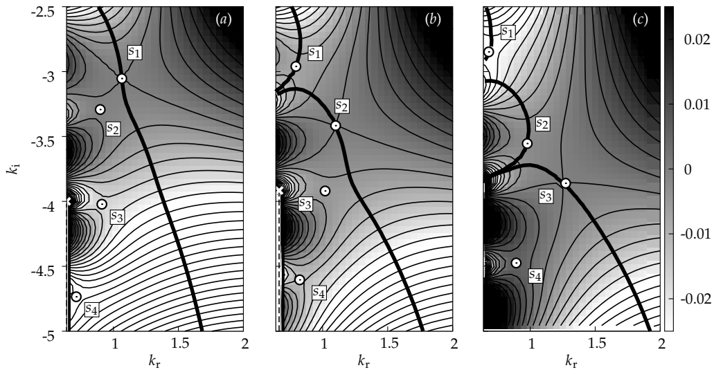
FIGURE 7. Zoom of the bottom-left corner of figure 6 for the same value of Re_z , three eccentricities around e \approx 0.3 and their associated critical Re_\Omega ; (a) e = 0.285 , Re_\Omega = 471.65 , s_1 is the dominating pinch; (b) zoom of previous figure, s_2 dominates; (c) e = 0.33 , Re_\Omega = 468.00 , s_3 dominates.
