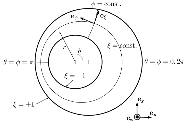
FIGURE 2. Modified bipolar coordinate system (\xi, \phi) fitting the eccentric annular domain. Polar coordinates (r, \theta) are centered on the inner cylinder, with \theta = \phi = 0 along the line joining the cylinder axes.
