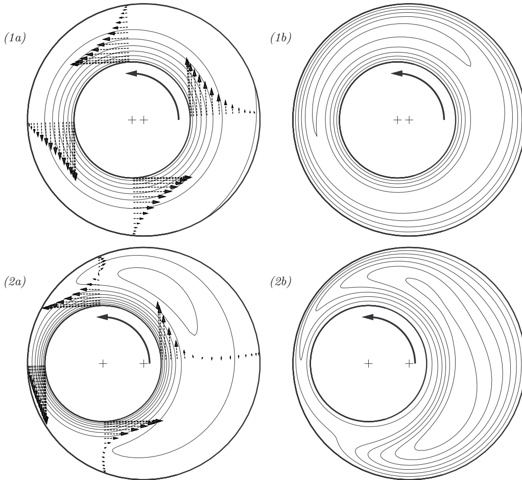
FIGURE 3. Basic flows for Re_\Omega = 500 : (1) weak eccentricity e = 0.2 , (2) high eccentricity e = 0.7 . (a) Contours of equispaced in-plane streamfunction with superimposed \mathbf{U}_\perp profiles at \theta = 0, \pi/2, \pi, 3\pi/2 (polar angle with respect to the inner cylinder). (b) Equispaced contours of W .
