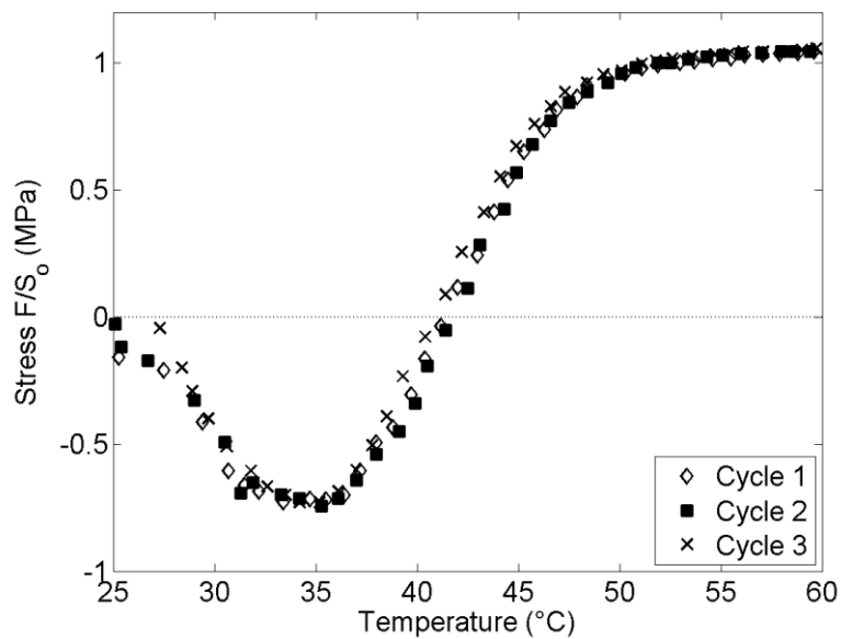
Figure 4: Step 4 constrained recovery during consecutive thermomechanical cycles for a sample pre-strained 20% at 65°C and heated at 5 °C/min.
