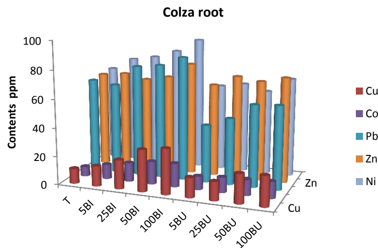
Figure 6: Distribution of heavy metals in the root of colza in soils with addition (5t/ha, 25t/ha, 50t/ha and 100t/ha) of urban (BU) and industrial (BI) sludge and control soil (T).
