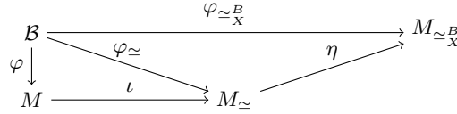
Fig. 2. Minimal strong recogniser.
