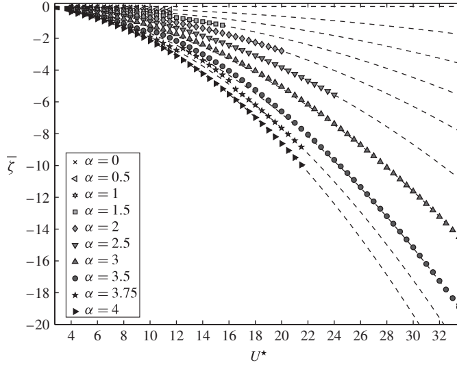
FIGURE 5. Time-averaged displacement as a function of the reduced velocity. For each rotation rate, a dashed line indicates the displacement induced by the time-averaged cross-flow force issued from the rigidly mounted cylinder case, as plotted in figure 4(b).
