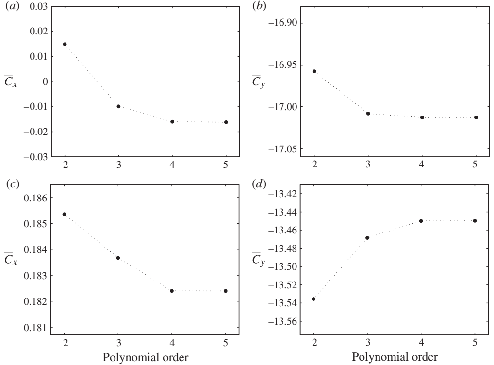
FIGURE 3. Time-averaged (a,c) in-line and (b,d) cross-flow force coefficients as functions of the polynomial order, for (a,b) a rigidly mounted rotating cylinder at \alpha=4 and (c,d) a flexibly mounted rotating cylinder at (\alpha, U^*) = (3.75, 13) at Re = 100 .
