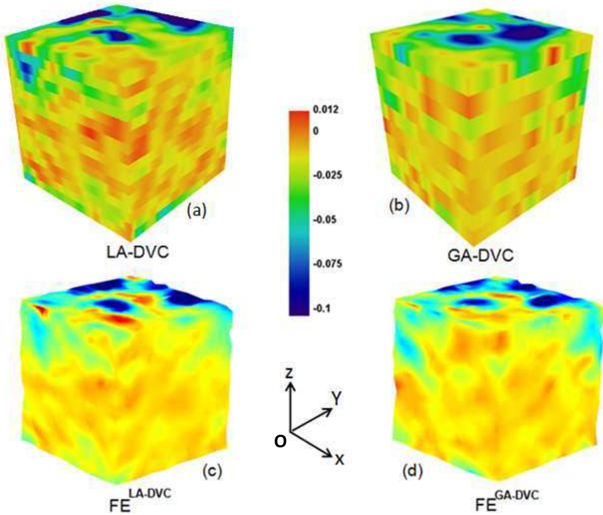
Fig.14. 3D visualization of the vertical strain, \varepsilon_{zz} , of the VOI (Fig. 4): (a) LA-DVC (sub-volume size: 0.64 mm with 50% overlap), (b) GA-DVC (element size: 0.64 mm), (c) FE model with boundary conditions applied from LA-DVC (average mesh size: 0.42 mm), (d) FE model with boundary conditions applied from GA-DVC (average mesh size: 0.42 mm). The macroscopic strain was applied along (Oz) direction.
