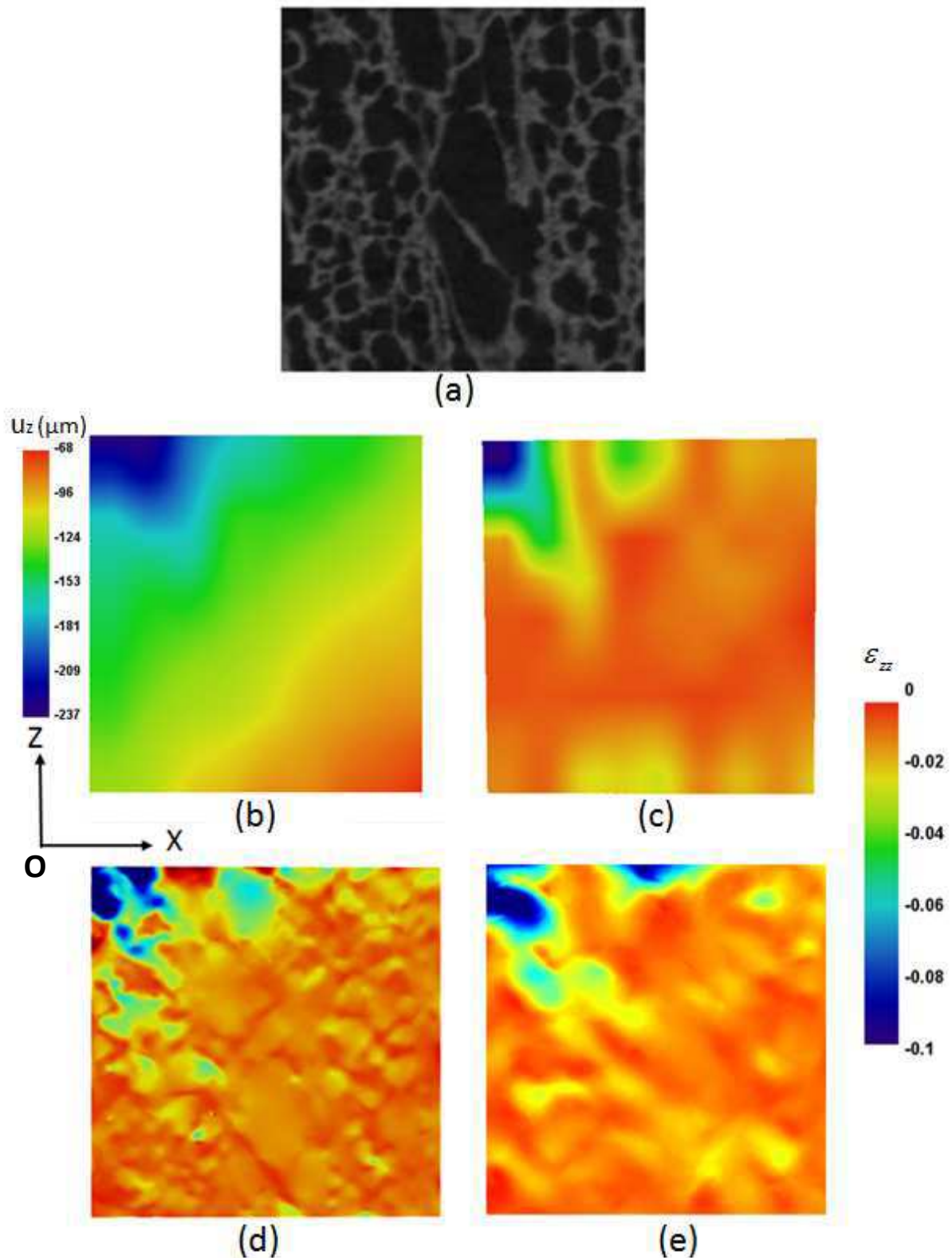
Fig. 15. Comparison of vertical strain magnitude, \varepsilon_{zz} , from DVC and FE model in a 2D section extracted from the core of the VOI (Fig. 4): (a): The micro-CT image, (b) u_z : DVC (sub-volume size: 0.64 mm), (c) \varepsilon_{zz} : DVC (sub-volume size: 0.64 mm), (d) \varepsilon_{zz} : FE model (average mesh size: 0.127 mm), (e) \varepsilon_{zz} : FE model (average mesh size: 0.42 mm). The macroscopic strain was applied along (Oz) direction. Similar maps were obtained for LA-DVC and GA-DVC and, for the sake of clarity, only LA-DVC is represented. The DVC maps were obtained with 50% overlap and a bicubic interpolation.
