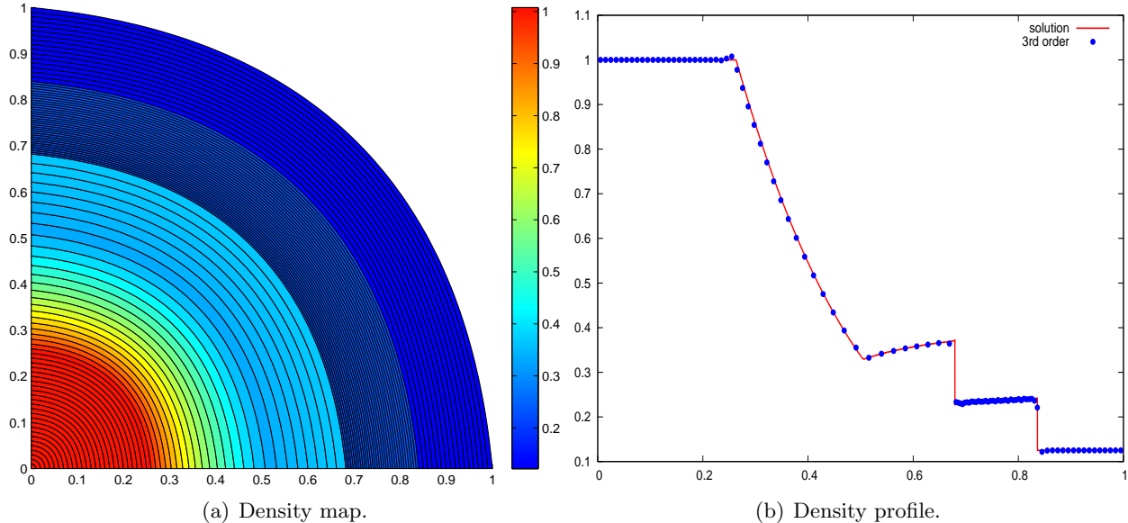
Figure 16: Polar Sod shock tube problem. Solution obtained with the third-order DG scheme without limitation on the domain defined in polar coordinates by (r, \theta) \in [0, 1] \times [0, \frac{\pi}{2}] made of 100 \times 1 cells.
