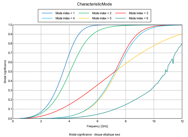
Figure 3: Modal significance of an elliptical disc 15×13 mm.
