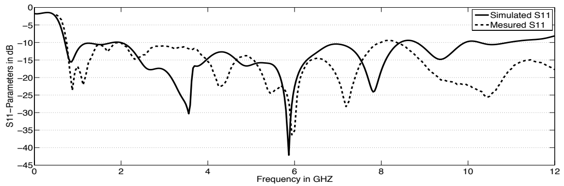
Figure 13: Comparison between simulated and measured S11
