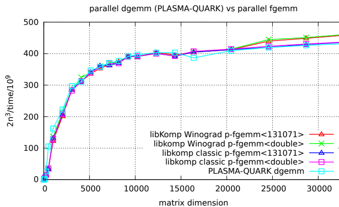
Figure 2: Comparison of execution time exact vs numeric
