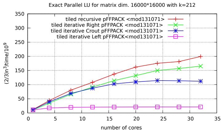
Figure 3: Parallel LU factorization on full rank matrices with modular operations
