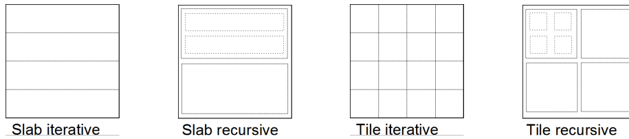
Figure 1: Main types of block splitting
