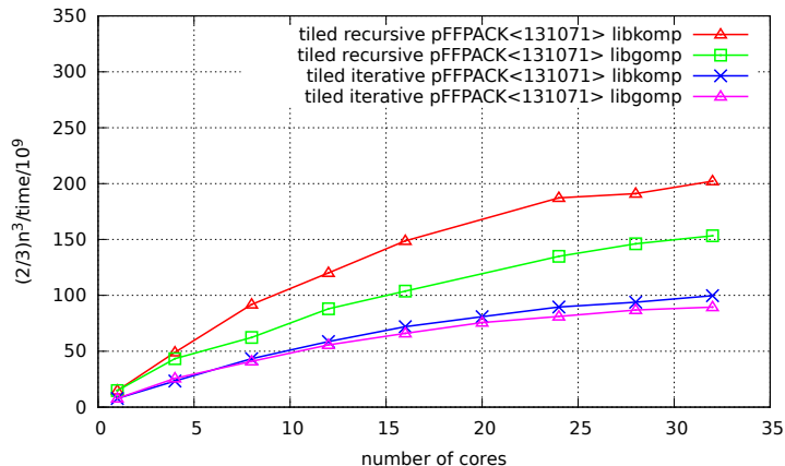
Figure 7: Performance of tiled recursive and tiled iterative factorizations using libgomp and libkomp . Matrix dimension n = 16000 with rank 15500
