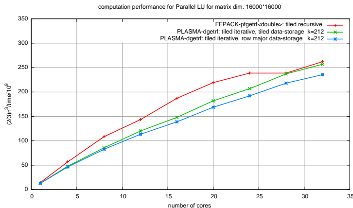
Figure 4: Parallel LU factorization on full rank matrices without modular operations
