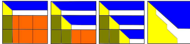
Figure 5: Slab iterative factorization of a matrix with rank deficiencies
