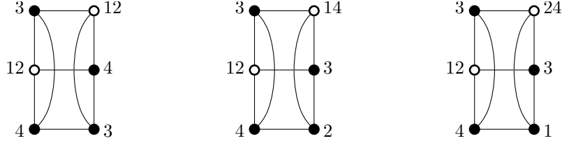
Figure 2: Valid colourings of Y_0 such that the pattern at X_0 is 12·3·4. The colouring of Y_0 is represented in the induced subgraph of H_n on C_0 \cup C_1 by assigning a pair of colours to each vertex in W . These vertices are shown as circles, the other vertices as solid dots.
