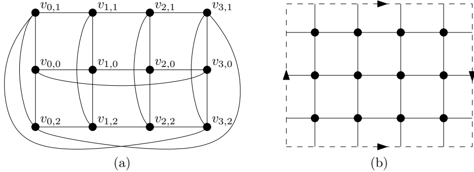
Figure 1: (a) The graph H_4 . (b) A drawing of H_4 as a quadrangulation of the Klein bottle. The opposite sides of the bounding rectangle are identified in such a way that the arrows match.
