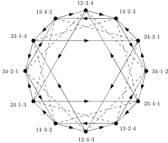
Figure 3: The auxiliary graph D . Directed loops at all the vertices are not shown.
