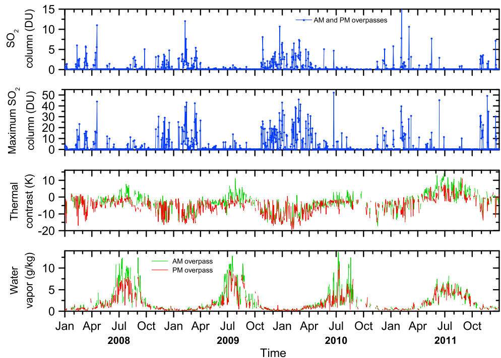
Figure 3. (first panel) Daily average retrieved \text{SO}_2 columns (0–2 km), expressed in DU; (second panel) daily maximum \text{SO}_2 columns (0–2 km, DU); (third panel) daily average thermal contrasts, calculated as the difference between the surface temperature and the temperature at 350 m above the ground; (fourth panel) daily average water vapor amount at 350 m, expressed in g/kg. All averages have been calculated for data in a circle of 50 km radius centered on Norilsk, for the period 1 January 2008 to 31 December 2011. Data from morning and evening IASI overpasses have been simultaneously averaged for \text{SO}_2 columns and the distinction is made for the thermal contrast and water vapor. Note that some measurements are missing for some days. They correspond to gaps in the data or cloudy scenes and have therefore been filtered.
