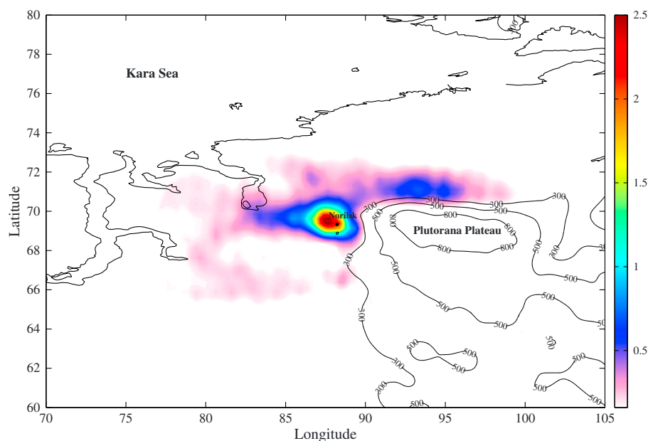
Figure 2. Distribution of the average retrieved 0–2 km \text{SO}_2 columns over the Norilsk region for February 2009, expressed in Dobson units. The average has been performed on a 0.25^\circ \times 0.25^\circ grid and then interpolated. The contour on the plot shows the terrain height in meters.
