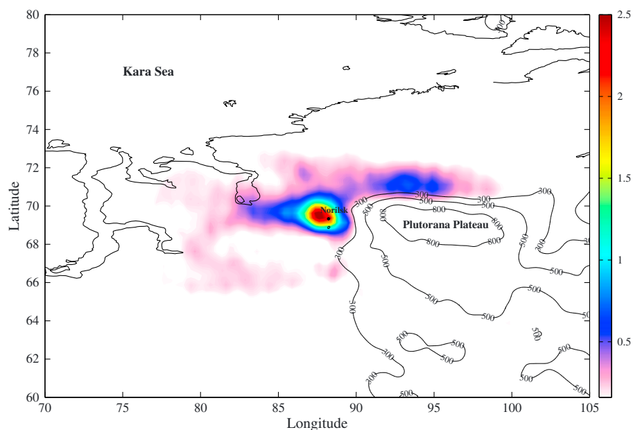
Figure 2. Distribution of the average retrieved 0–2 km SO 2 columns over the Norilsk region for February 2009, expressed in Dobson units. The average has been performed on a 0.25^\circ \times 0.25^\circ grid and then interpolated. The contour on the plot shows the terrain height in meters.
