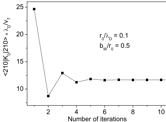
FIG. 1: Diagonal matrix element of K_0 for Ly- \alpha in terms of the number of iterations for r_0/\lambda_D = 0.1 , assuming b_W/r_0 = 0.5 . The calculation converges after only a few iterations.
