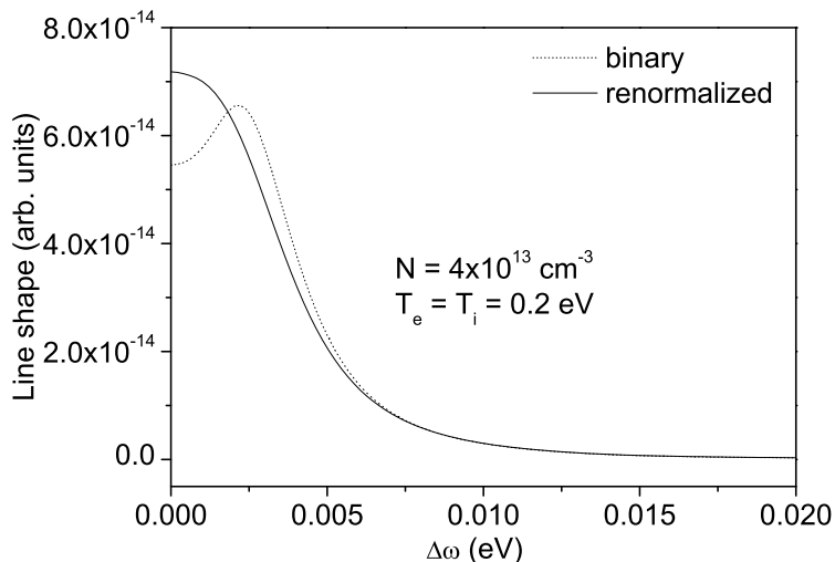
FIG. 3: Profile of \text{Ly}_{20} in recombining divertor plasma conditions. The dip present at the center stems from the neglect of correlated collisions. No dip is present if the renormalized model is used.
