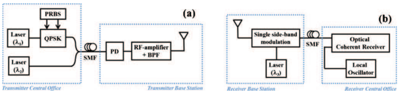
Fig. 9 Adopted architecture in the numerical simulation. Downlink (a) and uplink (b). PRBS , pseudo-random binary sequence; QPSK , quadrature phase shift keying; SMF , single mode fibre; PD , photodetector; RF , radio frequency; BPF , band-pass filter
