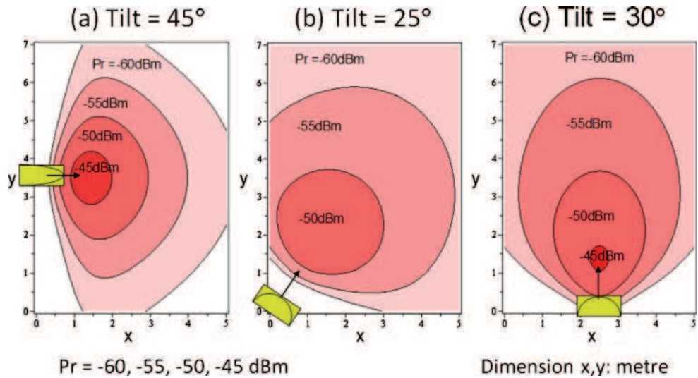
Fig. 4 Simulated wireless coverage ( P_r level) of a 60-GHz foam antenna for different positions in the horizontal plane ( x, y ) and different values of the tilt angle (from the ceiling plane): 45° (a), 25° (b), 30° (c)
