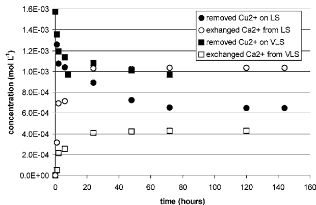
FIGURE 7. Evolution of Cu 2+ removed (mol/L) and Ca 2+ exchanged (mol/L) during kinetic experiment with carbonized sludges at 600 °C.
