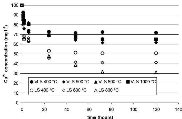
FIGURE 6. Adsorption kinetic of Cu 2+ onto carbonized sludges.
