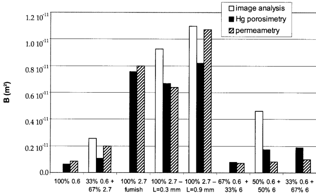
Figure 4. Permeability coefficients obtained from equation (ix) from mercury porosimetry and image analysis experiments: comparison with air permeametry measurements.
