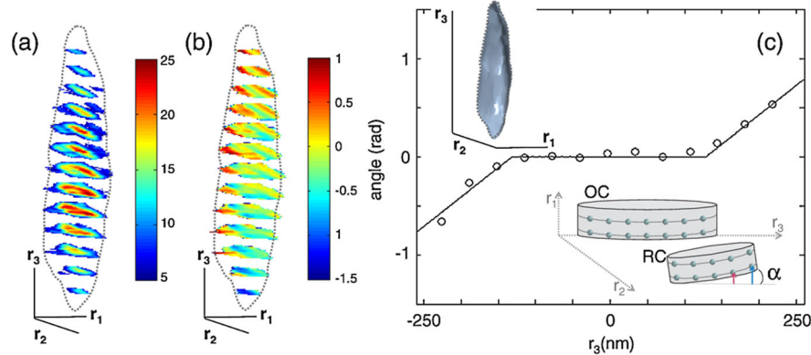
FIG. 4 (color online). Stack of 2D slices extracted from the 3D direct space matrix. (a) Internal view of the object image density [the color scale is linear (arbitrary unit)] and (b) phase (the angular color scale is given in radians). (c) Mean values of the object image phases (black circles) as a function of r_3 (in nm), calculated from (b); expected phase behavior (solid line) calculated for a RC density function with linear phase shift. This phase behavior results from a tilt ( \alpha ) of the RC lattice planes with respect to OC. The inset at the bottom shows two values of \mathbf{u}_{004} (pink and blue arrows), which increases linearly with \mathbf{r}_3 when the RC is tilted.
