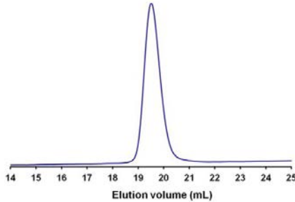
Figure 1: Typical size exclusion chromatography (SEC) curve of a PS- b -PMMA BCP, synthesized on an industrial scale, exhibiting a molecular chain dispersity of 1.07.
