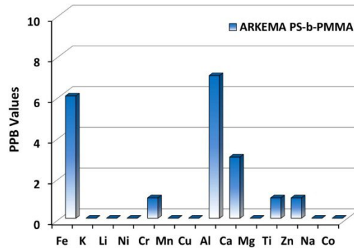
Figure 3: ICP-MS study showing the low metallic contamination level of PS- b -PMMA BCPs after purification.
