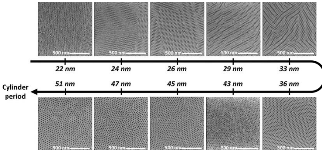
Figure 4: SEM top-view pictures illustrating perpendicular self-assembly of various PS- b -PMMA cylindrical BCPs (PMMA cylinders in a PS matrix) with periods ranging from 22 nm up to 51 nm.
