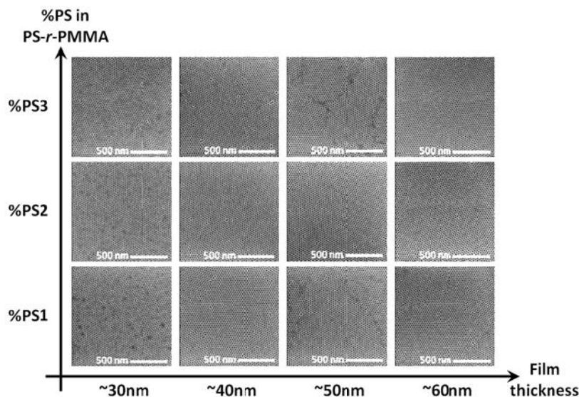
Figure 7: Self-assembly of a BCP with different film-thickness on various PS- r -PMMA with different PS contents showing that weak surface-energy dependence may be achieved.
