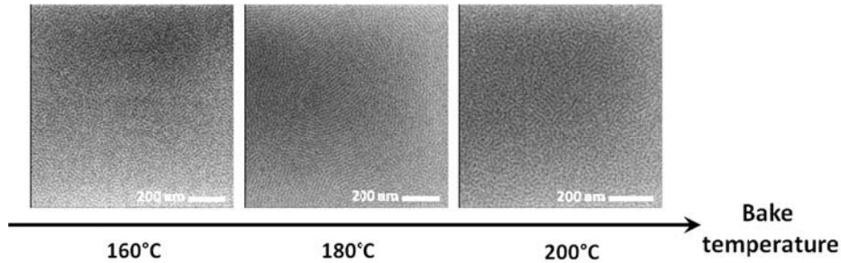
Figure 8: Self-assembly of a low molecular weight lamellar PS- b -PMMA BCP presenting a T_{ODT} close to 190°C, illustrating the fact that the process parameters must be carefully tuned to reach an optimal order.
