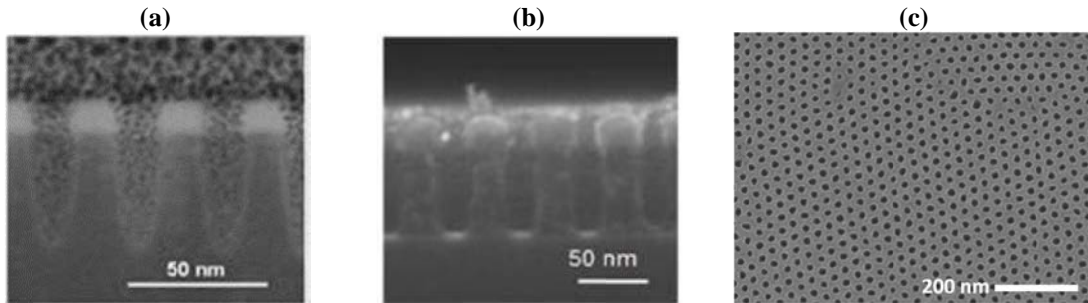
Figure 9: Left and middle pictures: 36 nm-period BCP transferred in bulk silicon and SOC substrate respectively (the upper white areas are the remaining SiO 2 and SiARC hard-masks respectively). Right picture: 10 nm-thick silica hard-mask after dry etch-transfer of a PS- b -PMMA BCP leading to features with CD close to 11 nm.
