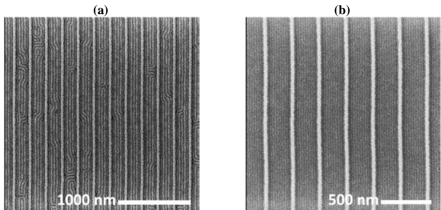
Figure 10: Graphoepitaxy of two lamellar BCPs having different molecular weights, illustrating the increase in ordering for a low molecular weight BCP (b) when the same self-assembly process with a higher molecular weight (a) one is done (white lines: HSQ template).
