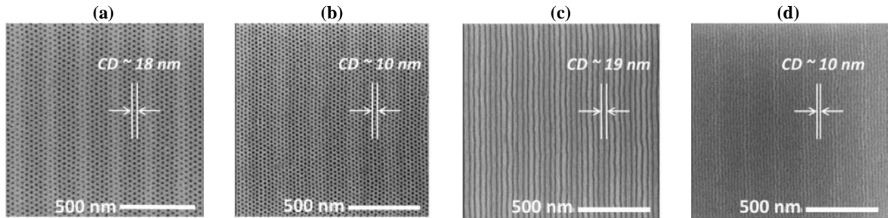
Figure 11: Macroscopic-sized BCPs crystals obtained from a high molecular weight cylindrical BCP (a) and a low molecular weight cylindrical BCP (b), a high molecular weight lamellar BCP (c) and a low molecular weight lamellar BCP (d) (lighter grey areas: BCPs above the HSQ-resist lines).
