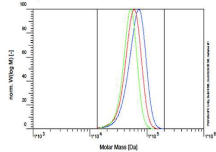
Figure 2: GPC curves of three BCPs with different molecular weights, synthesized from the same PS-living block.
