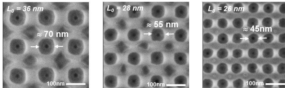
Figure 12: Various pre-patterned contact-hole sizes shrunk with different PS- b -PMMA BCPs having periods of 36, 28 and 26 nm respectively.
