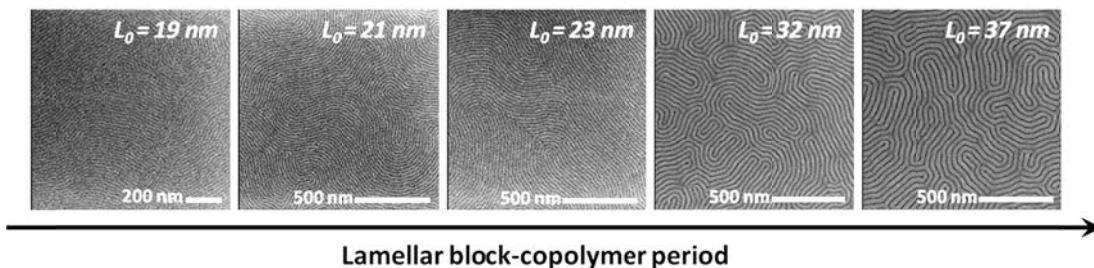
Figure 5: SEM pictures showing the perpendicular self-assembly of lamellar BCPs with periods ranging from 19 nm up to 37 nm.
