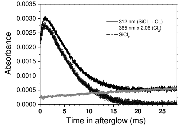
Figure 2. Time variation of the absorbance measured at 312 nm (which includes contributions from Cl 2 and SiCl 2 ) and at 365 nm (Cl 2 alone). The absorbance at 365 nm has been multiplied by 2.06 to account for the difference in the Cl 2 absorption cross sections at 365 and 312 nm. The time variation of the SiCl 2 density (dotted curve) has been obtained by subtracting the Cl 2 contribution from the absorbance at 312 nm. Plasma conditions: Ar (100 sccm)/Cl 2 (100 sccm)/SiCl 4 (60 sccm) at 10 mTorr with 800 W RF power pulsed at 30 Hz with 15 % duty cycle.
