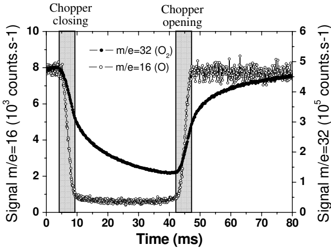
Figure 7. MS signals versus time during the closing and the opening of the chopper at m/e = 16 with an electron energy set at 15 eV (O radical) and at m/e = 32 at 25 eV. Plasma conditions: 10 mtorr O_2 pressure, 800 W RF ICP power. The shaded area indicates the time windows during which the chopper opens and closes.
