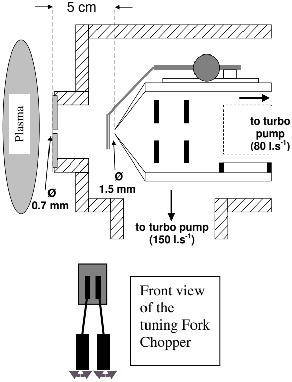
Figure 4. Schematic of the mass spectrometer head (modified hidden EQP 500) with the tuning fork chopper fitted on the top of the MS ionization chamber.
