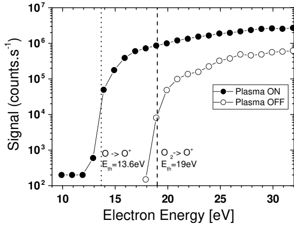
Figure 6. MS signals at m/e = 16 (O atoms) versus electron energy with the plasma on and off. Plasma conditions: 10 mtorr O_2 pressure, 800 W RF ICP power.
