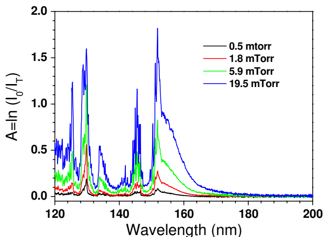
Figure 3. VUV absorption spectrum of \text{Cl}_2 gas at different pressures without plasma.
