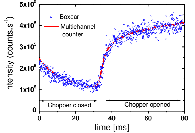
Figure 5. MS signals versus time during the opening of the chopper at m/e = 40 in pure Ar gas at 5 mTorr. Open symbols: data with a boxcar, solid line: data for the same acquisition time with a multichannel counter.
