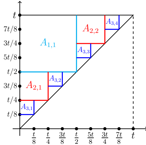
FIGURE 1. Le Gall's partition of T_2(t) into disjoint rectangles of decreasing area.
