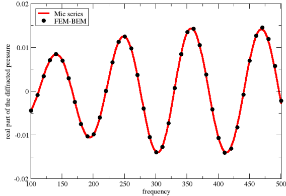
Figure 4: Zero flow: Real part of the scattered pressure at the sensor in function of the frequency (validation of the FEM-BEM on the sphere test case).
