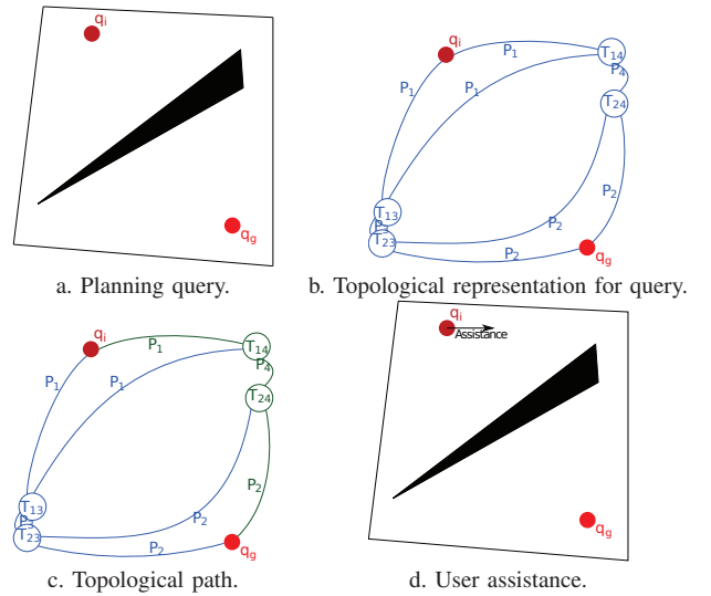
Fig. 6. Environment representation for interactive path planning.
