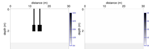
Figure 4: Near-surface test case pressure wave velocity models, exact (left), initial (right)
