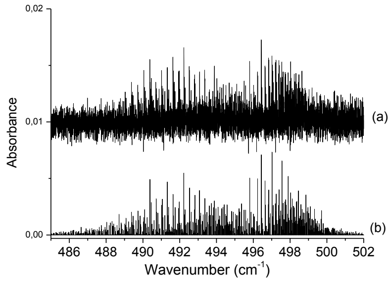
Figure 5: Global view of the Jet-AILES \nu_6 spectrum recorded at 0.005 \text{ cm}^{-1} resolution (a) and our best simulation at T_{rot} = 30 \text{ K} (b).
