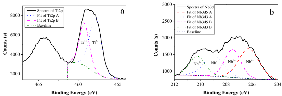
Fig. S10. High resolution XPS spectra of Ti (a) and Nb (b) of the 10 % at Nb-TiO 2 HTR fibres.
