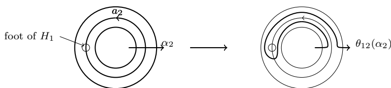
Figure 16: Action of \theta_{12} on \alpha_2
