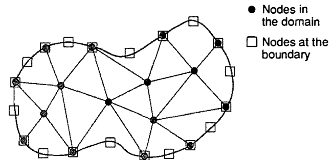
Fig. 3—Discretization.
