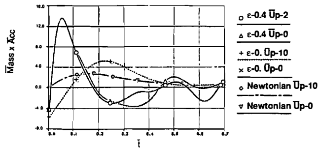
Fig. 15—Mass \times Acceleration, \bar{m} = 81.5 , \bar{W}_{imposed} = 1 ; Newtonian fluid, MPTT fluid W_f = 0.4 , \beta = 0.5 , n = 1 , \xi = 0 , \xi = 0 and \xi = 0.4 .
