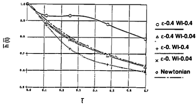
Fig. 9— h(\bar{t}) , \bar{m} = 81.5 , \bar{W}_{imposed} = 1 ; MPTT Fluid.
