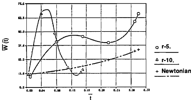
Fig. 8—Influence of L/h_0 parameter. MPTT Fluid: W_i = 0.4 , \xi = 0.4 , \beta = 0.5 , n = 1 , \varepsilon = 0 , L/h_0 = 5 , L/h_0 = 10 .
