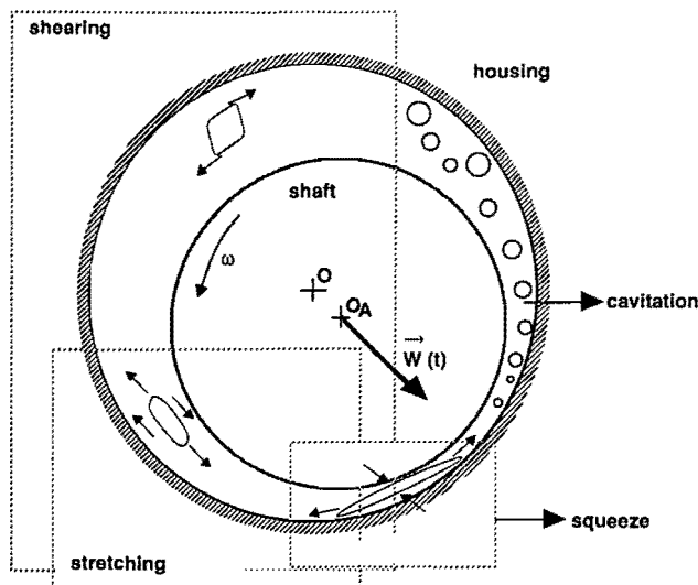
Fig. 4—Solutions in a journal bearing in the case of overloading.
