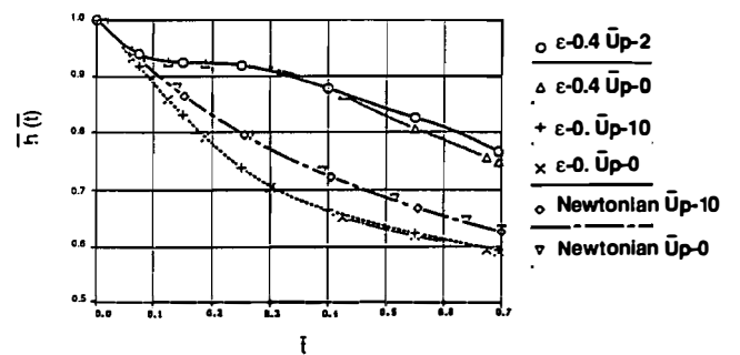
Fig. 14— h(\bar{t}) , \bar{m} = 81.5 , \bar{W}_{imposed} = 1 ; Newtonian fluid, MPTT fluid W_i = 0.4 , \beta = 0.5 , \eta = 1 , \epsilon = 0 , \xi = 0 and \xi = 0.4 .
