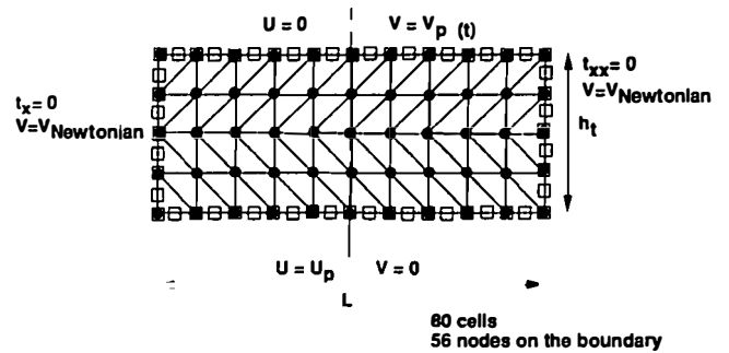
Fig. 13—Domain of study and boundary conditions.
