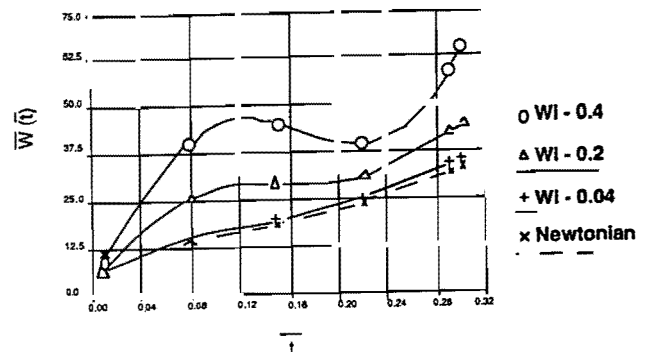
Fig. 6—Influence of Weissenberg number. MPTT Fluid: \xi = 0.4 , \beta = 0.5 , \epsilon = 0 , n = 1 , W_i = 0.04 , W_i = 0.2 , W_i = 0.4 .
