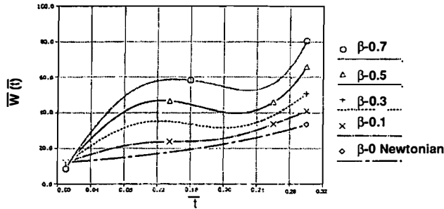
Fig. 7—Influence of \beta parameter. MPTT Fluid: W_i = 0.4 , \xi = 0.4 , n = 1 , \varepsilon = 0 , \beta = 0 , \beta = 0.3 , \beta = 0.5 , \beta = 0.7 .
