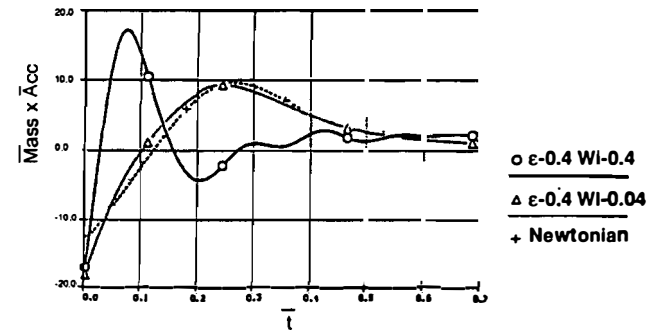
Fig. 12—Mass \times Acceleration = \bar{m} = 163 , \bar{W}_{imposed} = 2 ; MPTT Fluid.
