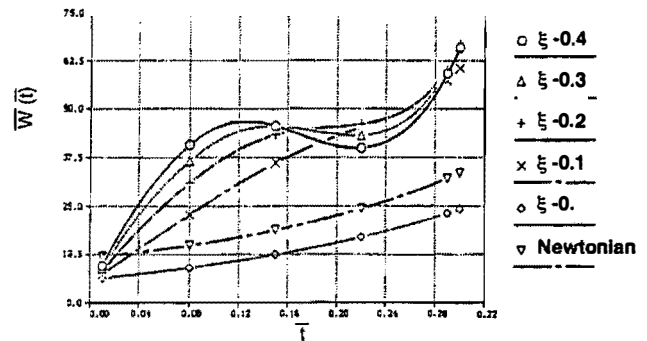
Fig. 5—Influence of \xi parameter. MPTT fluid: W_i = 0.4 , \beta = 0.5 , \epsilon = 0 , \xi = 0 , \xi = 0.1 , \xi = 0.2 , \xi = 0.3 , \xi = 0.4 .
