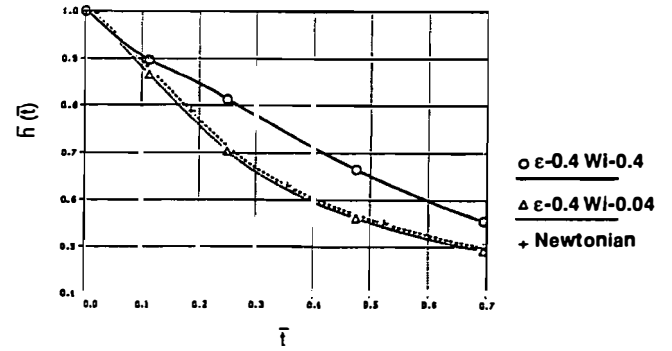
Fig. 11— h(\bar{t}) , \bar{m} = 163 , \bar{W}_{imposed} = 2 ; MPTT Fluid.
