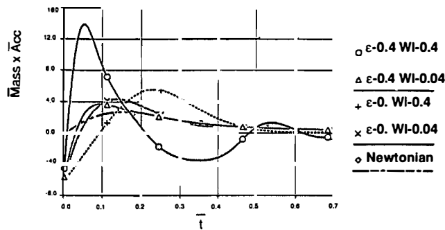
Fig. 10—Mass \times Acceleration = \bar{m} = 81.5 , \bar{W}_{imposed} = 1 ; MPTT Fluid.
