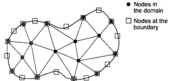
Fig. 3—Discretization.
