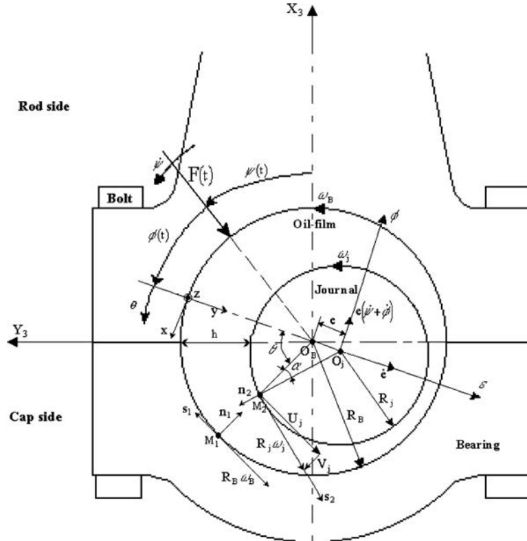
Fig. 1—Connecting rod big end journal bearing and coordinate system.
