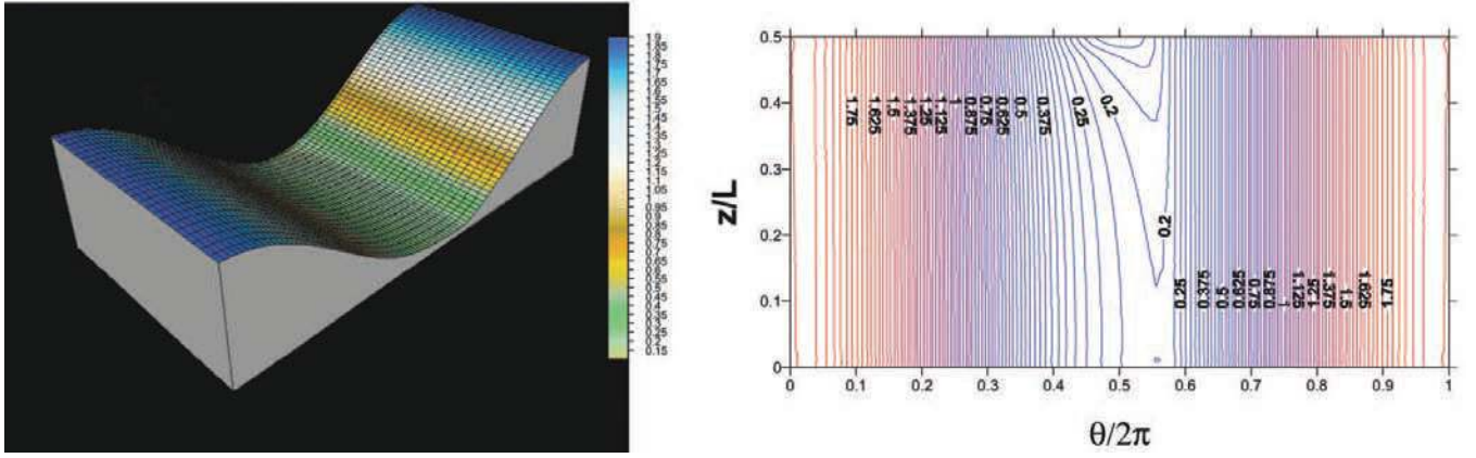
Fig. 7—Steady-state film thickness distributions for rigid and compliant journal bearings, \varepsilon_0 = 0.9 .
