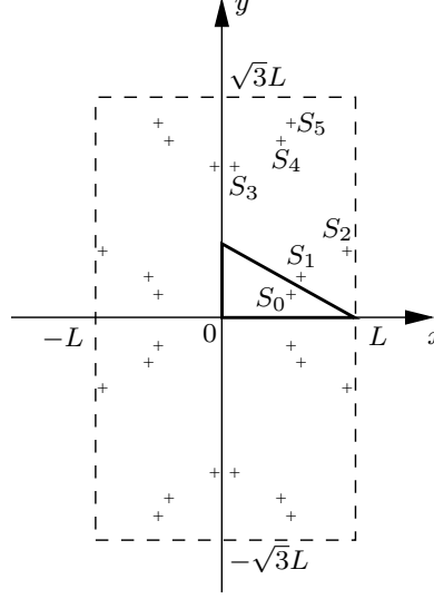
Figure 16: Elementary cell of the half-equilateral triangular plate. Six sources, denoted S_i ( i = 0, \dots, 5 ) and located at (x_i, y_i) , are necessary to describe this cell.
