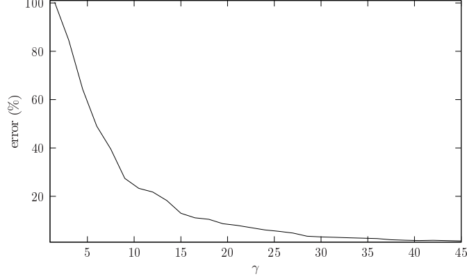
Figure 14: Error on the estimation of |G_\Omega| as a function of \gamma for the isosceles right triangular plate, averaged over the high-frequency band.
