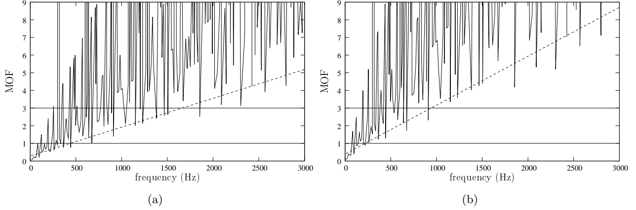
Figure 9: Modal Overlap Factor of the isosceles right triangular plate for two values of the structural damping ratio: (a) \eta = 3 \cdot 10^{-2} ; (b) \eta = 5 \cdot 10^{-2} . —, MOF; ----, least-squares fit of the local minimum.
