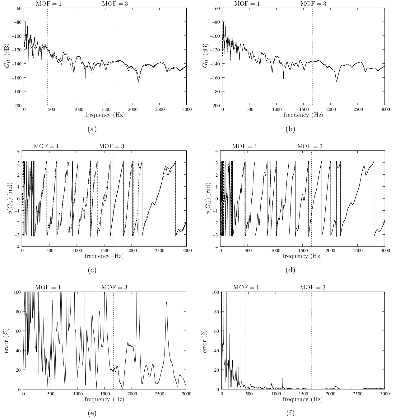
Figure 13: Frequency response of the isosceles triangular plate for two values of the truncation parameter: (a) modulus, (c) phase and (e) error for \gamma = 6.15 ; (b) modulus, (d) phase and (f) error for \gamma = 30.74 . —, exact solution; ----, AISM.
