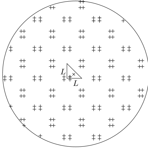
Figure 8: Image source cloud of the isosceles right triangular plate, for the truncation parameter \gamma = 10.76 ( r_t = 4.95 m), containing 154 sources.
