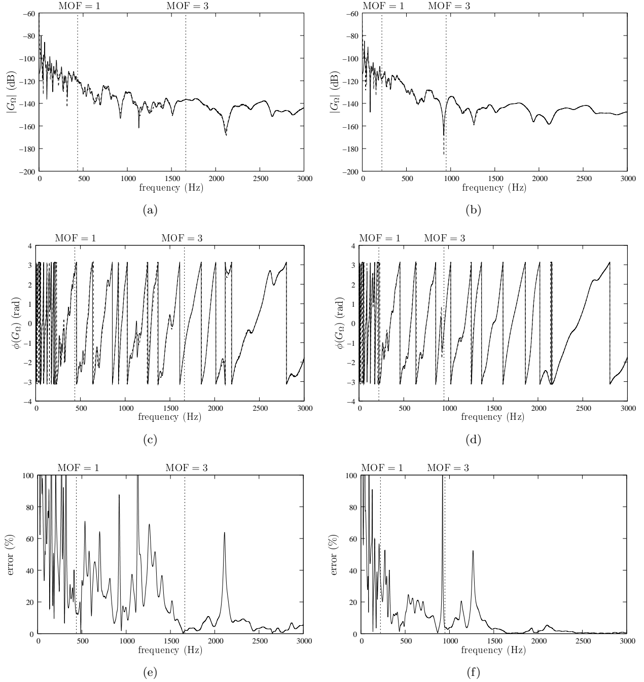
Figure 10: Frequency response function of the simply supported isosceles right triangular plate between source \mathbf{r}_0 and receiver \mathbf{r} , calculated by modal expansion and by AISM for the truncation parameter \gamma = 10.76 , for two values of the structural damping ratio: (a) modulus, (c) phase and (e) error for \eta = 3 \cdot 10^{-2} ; (b) modulus, (d) phase and (f) error for \eta = 5 \cdot 10^{-2} . —, exact solution; ----, AISM.
