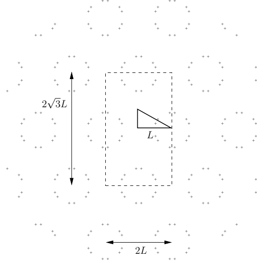
Figure 5: Image source cloud for the half-equilateral triangular plate. —, plate boundaries; +, sources; ----, elementary cell \mathcal{E} .
