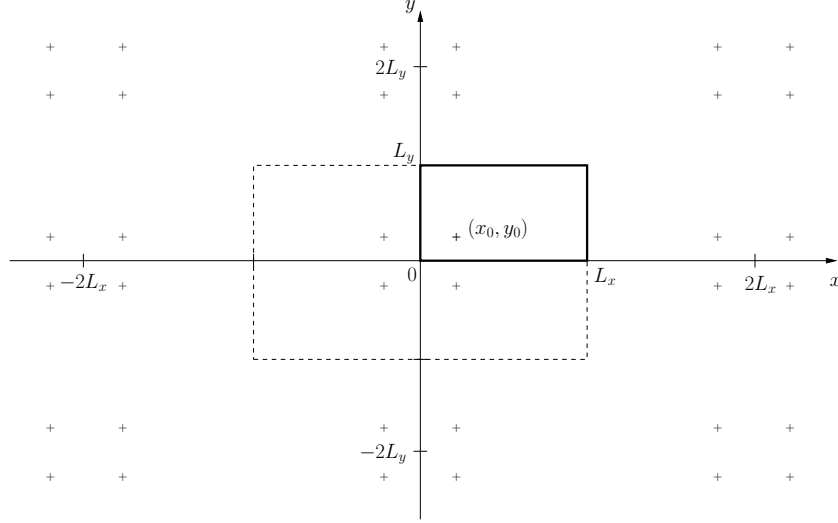
Figure 3: Image source cloud for a rectangular plate. —, plate boundaries; +, sources; ----, elementary cell \mathcal{E} .
