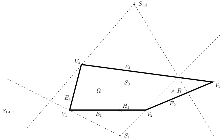
Figure 15: Example of image source geometrical construction. —, plate boundaries; +, sources; ×, receiver; ---, light zones limits.
