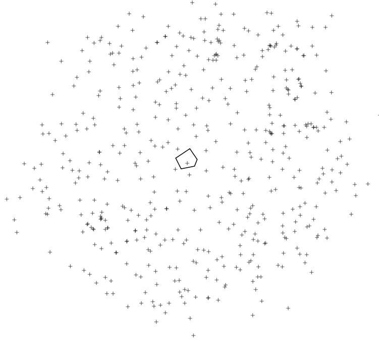
Figure 2: Image source cloud for an arbitrarily convex polygonal plate (first 12 reflections, giving rise to 483 image sources). —, plate boundaries; +, sources.
