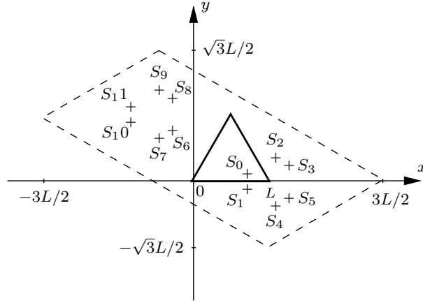
Figure 17: Elementary cell of the equilateral triangular plate. Twelve sources, denoted S_i ( i = 0, \dots, 11 ) and located at (x_i, y_i) , are necessary to describe this cell.
