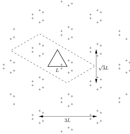
Figure 6: Image source cloud for the equilateral triangular plate. —, plate boundaries; +, sources; ----, elementary cell \mathcal{E} .
