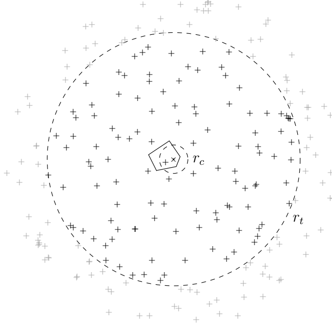
Figure 7: Example of image source cloud truncation for AISM. —, plate boundaries; ----, characteristic and truncation circles of radii r_c and r_t centered on the receiver; +, sources taken into account for AISM; +, ignored image sources.
