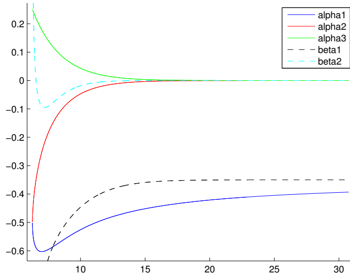
Figure 3: Here, we plot the characteristic velocities \{\alpha_j(X(k))\}_{j=1}^3 and \{\beta_j(X(k))\}_{j=1}^2 for the Whitham system for Korteweg-de Vries equation and the relaxed Whitham's system (4.34), respectively, as functions of the period X(k) of the underlying wave train.
